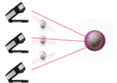
NetProfiler 3
